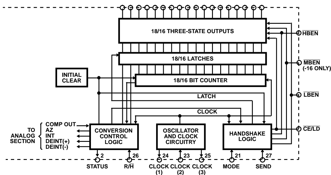
FIGURE 9. DIGITAL SECTION
