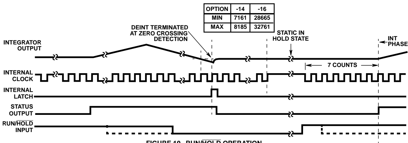
FIGURE 10. RUN/HOLD OPERATION
