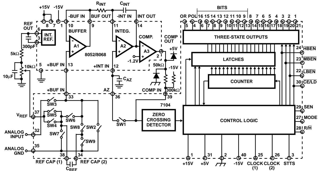
FIGURE 1. ICL8052A (8068A)/ICL7104 16-BIT/14-BIT A/D CONVERTER FUNCTIONAL DIAGRAM
