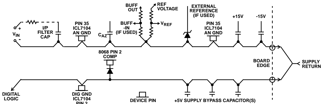
FIGURE 16. GROUNDING SEQUENCE
