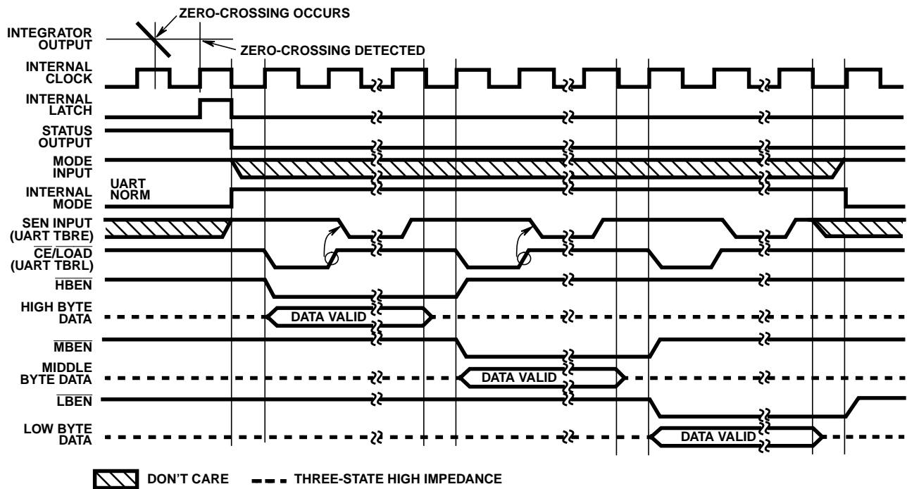
FIGURE 12. HANDSHAKE - TYPICAL UART INTERFACE TIMING
