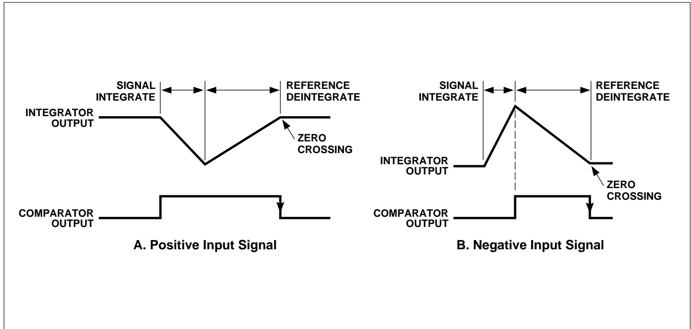
Figure 5. Comparator Output
